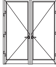
GU PVC KANALLI TEK EKSEN ÇİFT KANAT AÇILIM SETİ 100 kg GU DOUBLE SASH OPENING SET FOR PVC CHANNEL 100 kg KANAT YÜKSEKLİĞİ (H) MAX.2100MM SASH HEIGHT (H) MAX.2100MM
