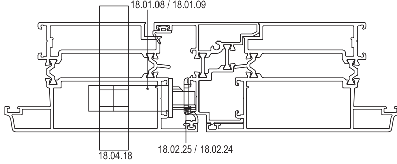
**PVC AKSESUARA UYGUN İÇE AÇILIM KAPI DETAYI **INWARD OPENING DOOR DETAIL FOR PVC ACCESSORIES
