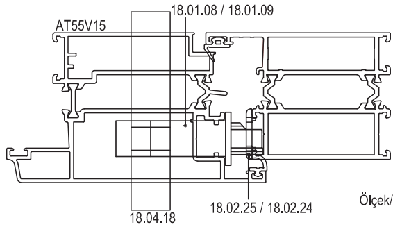
**PVC AKSESUARA UYGUN DIŞA AÇILIM KAPI DETAYI **OUTWARD OPENING DOOR DETAIL FOR PVC ACCESSORIES
