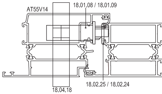
**PVC AKSESUARA UYGUN İÇE AÇILIM KAPI DETAYI **INWARD OPENING DOOR DETAIL FOR PVC ACCESSORIES
