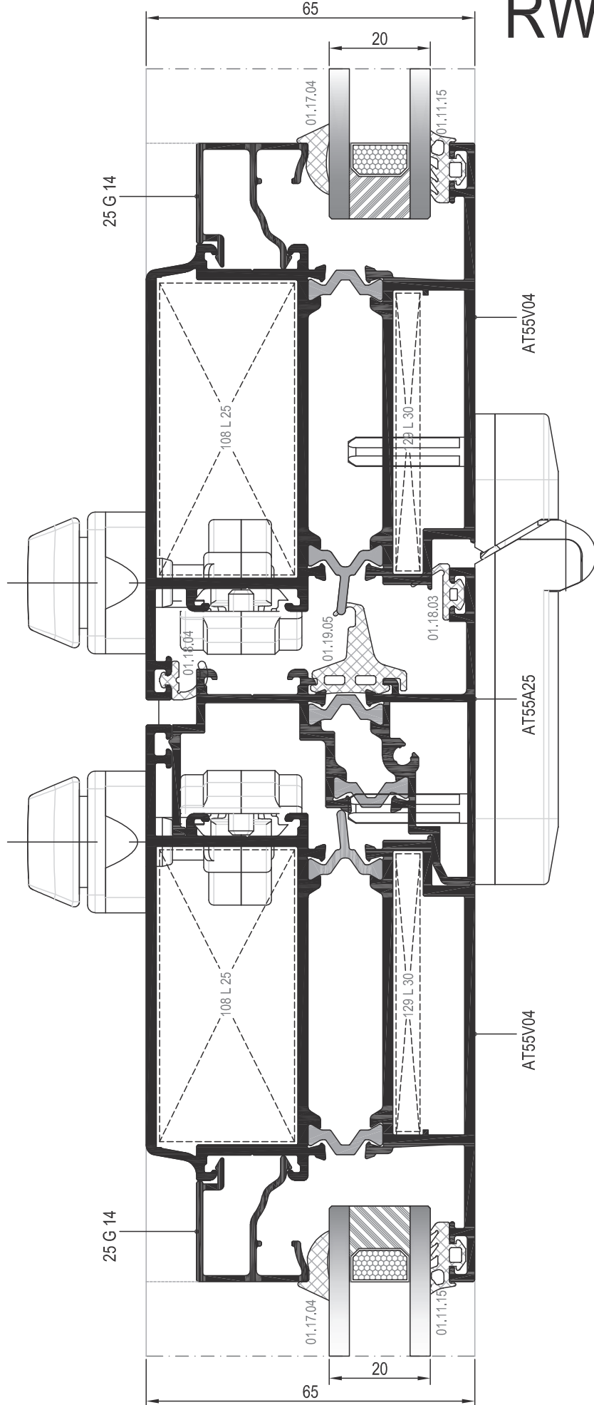
KATLANIR KAPI DETAYI FOLDING DOOR DETAILS
