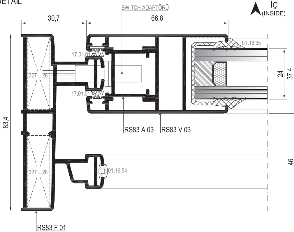
SWITCH DETAYI SWITCH DETAIL
