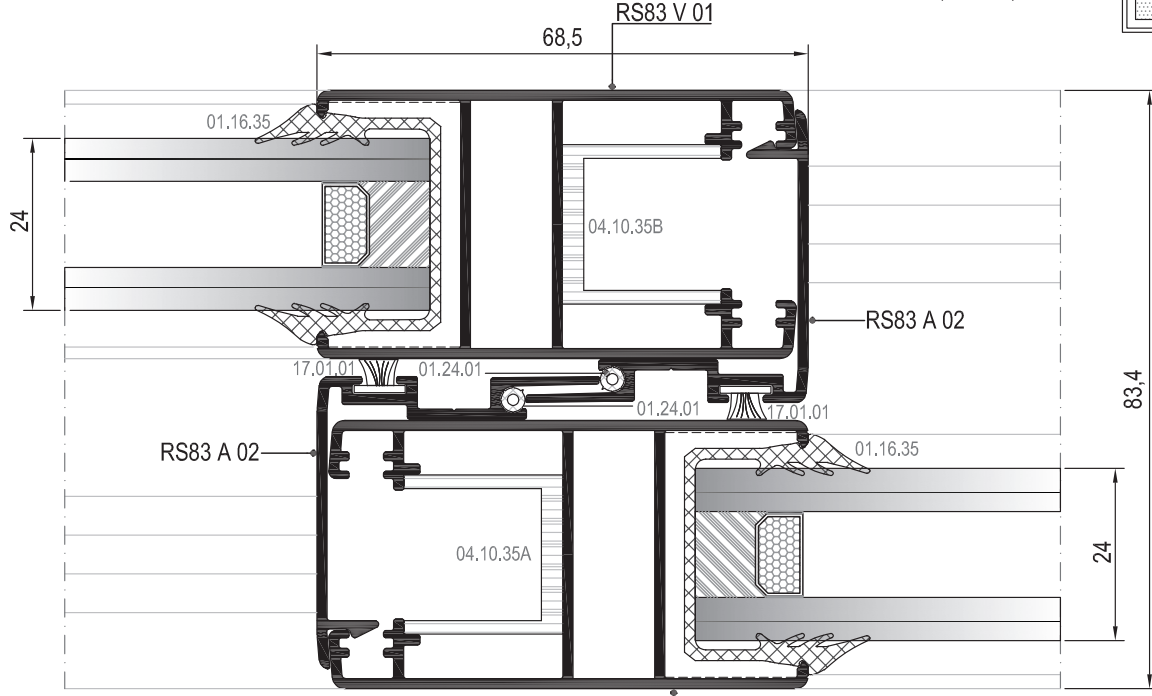
③ DETAYI DETAIL
